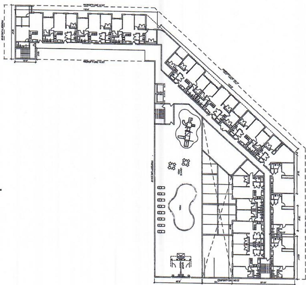
NORTH FIFTH FLOOR PLAN
