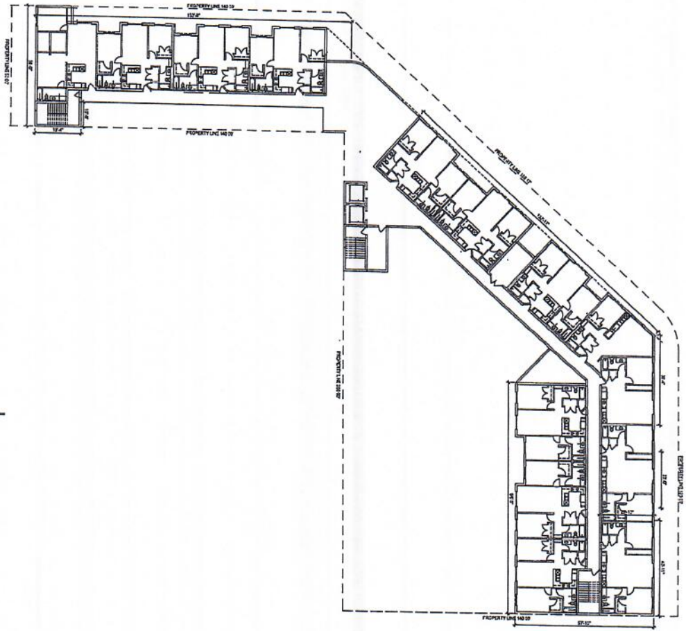
NORTH EIGHTH FLOOR PLAN
